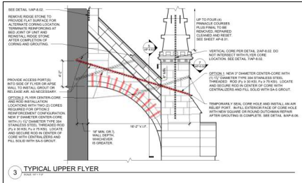
3 TYPICAL UPPER FLYER
